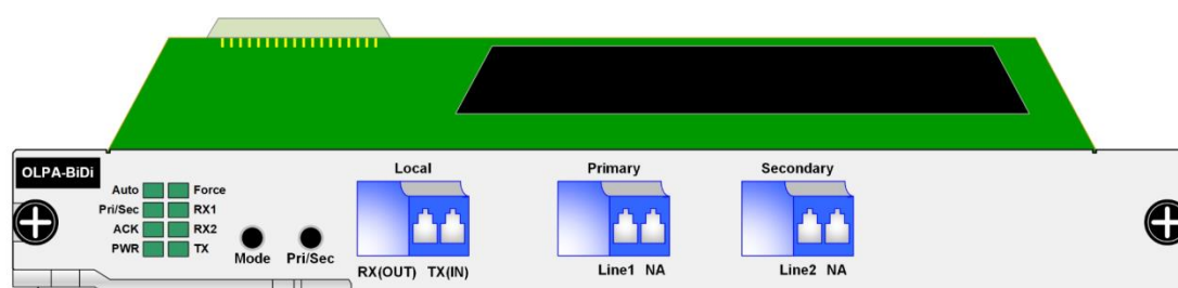
Figure 2.3.3-1 OLPA-BiDi board
